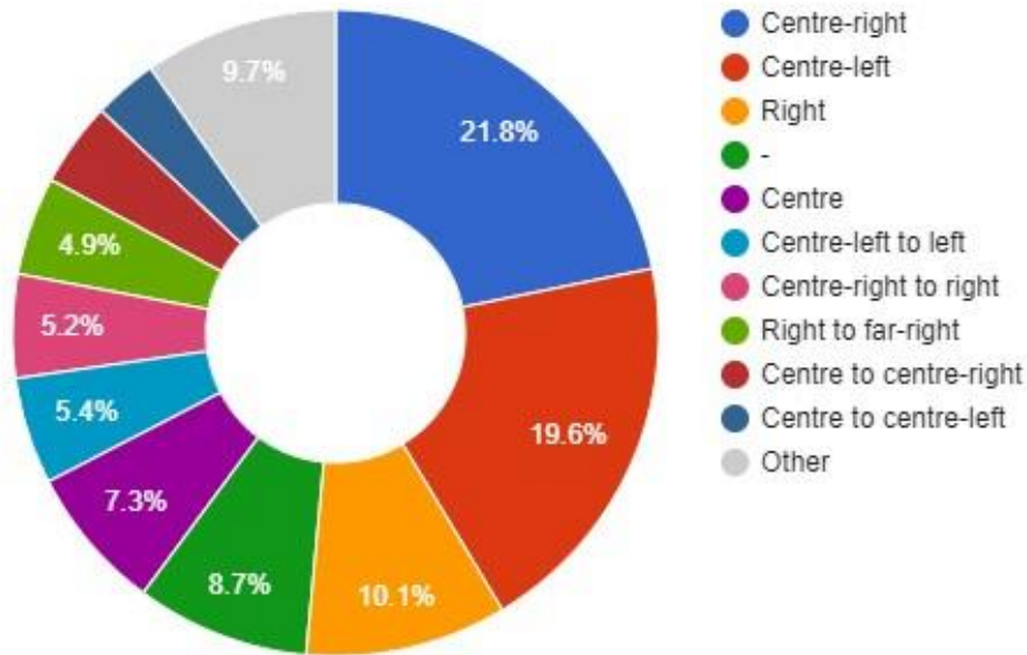
speech - party_orientation
