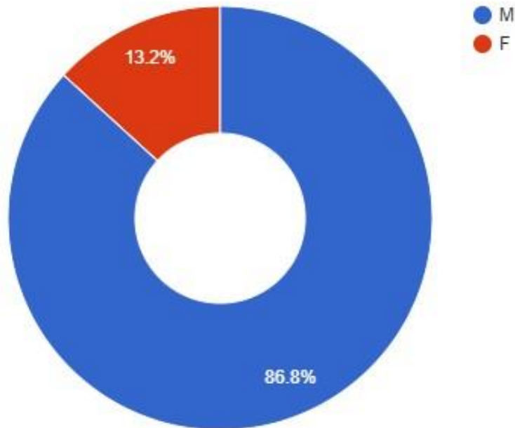
speech - speaker_gender
